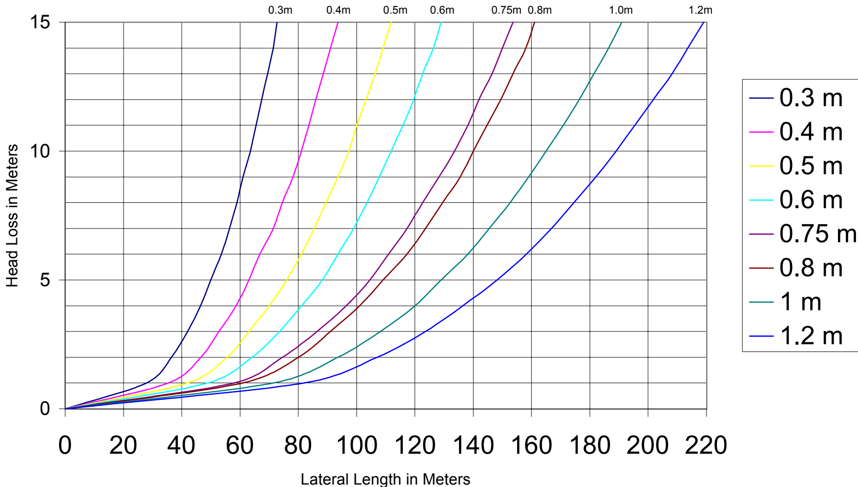
Lateral Head Loss Chart (0% Slop) Calculated for Various Spacing 12mm x 2.0 l/h
